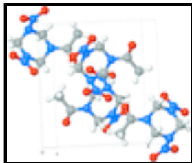
Fig. 2. The packing of the title compound, viewed down the c axis of the unit cell.
